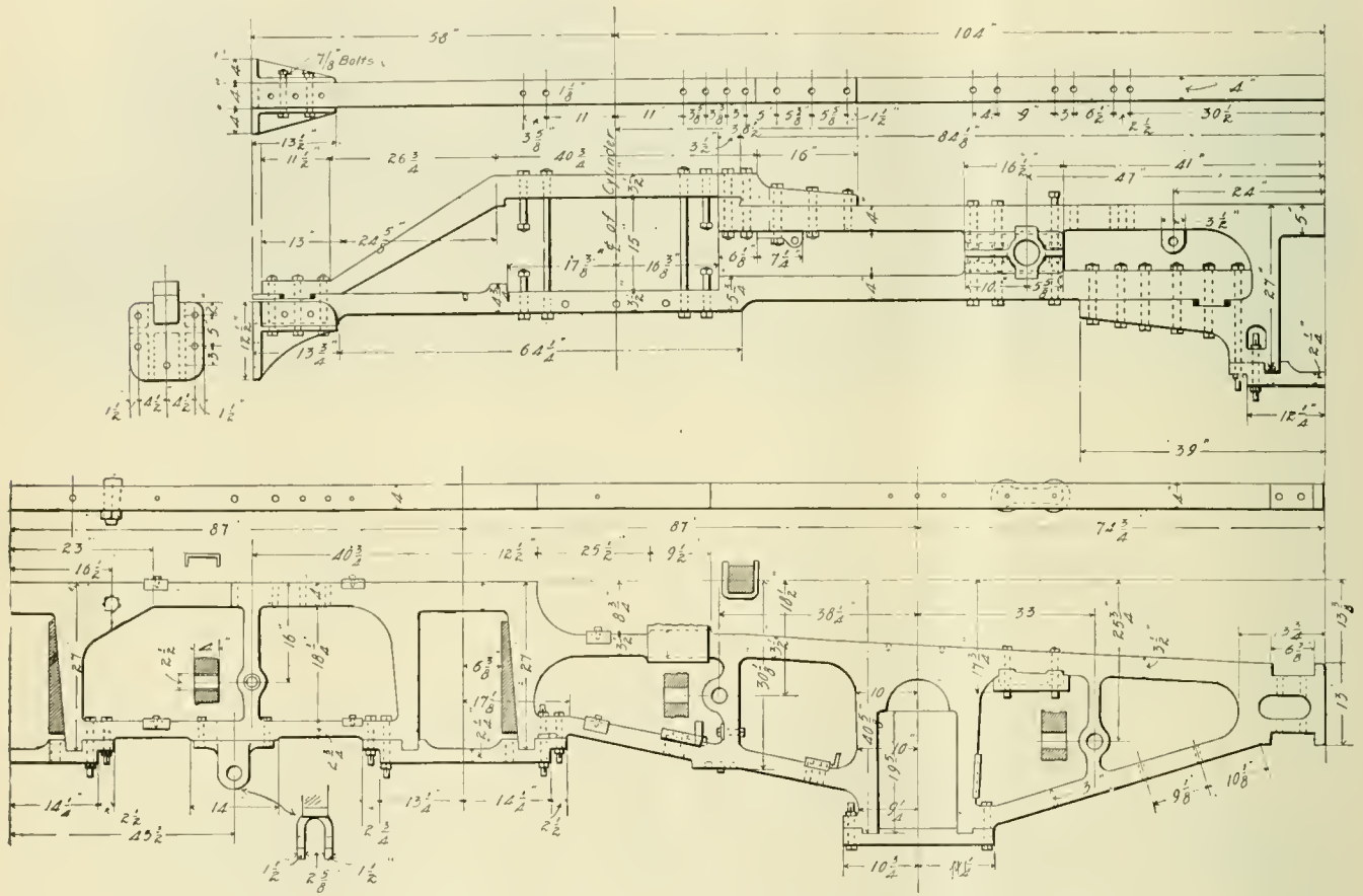
DETAIL OF FRAMES FOR ATLANTIC LOCOMOTIVE-CENTRAL OF NEW JERSEY.
